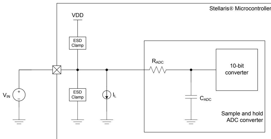
Figure 25-11. ADC Input Equivalency Diagram
